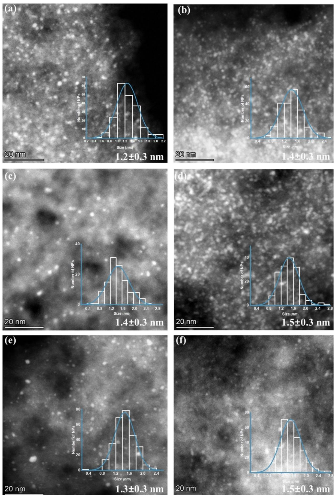
Figure S4. (a) HAADF-STEM image of Ru@AC; (b-f) HAADF-STEM images of Ru@SILP AC with fixed Ru loadings ( 0.1 \text{ mmol}_{\text{Ru}}\cdot\text{g}^{-1} theoretical) and varying IL loadings of (b) 0.5 \text{ mmol}\cdot\text{g}^{-1} ; (c) 0.8 \text{ mmol}\cdot\text{g}^{-1} ; (d) 1.1 \text{ mmol}\cdot\text{g}^{-1} ; (e) 1.7 \text{ mmol}\cdot\text{g}^{-1} ; (f) 2.4 \text{ mmol}\cdot\text{g}^{-1} .
