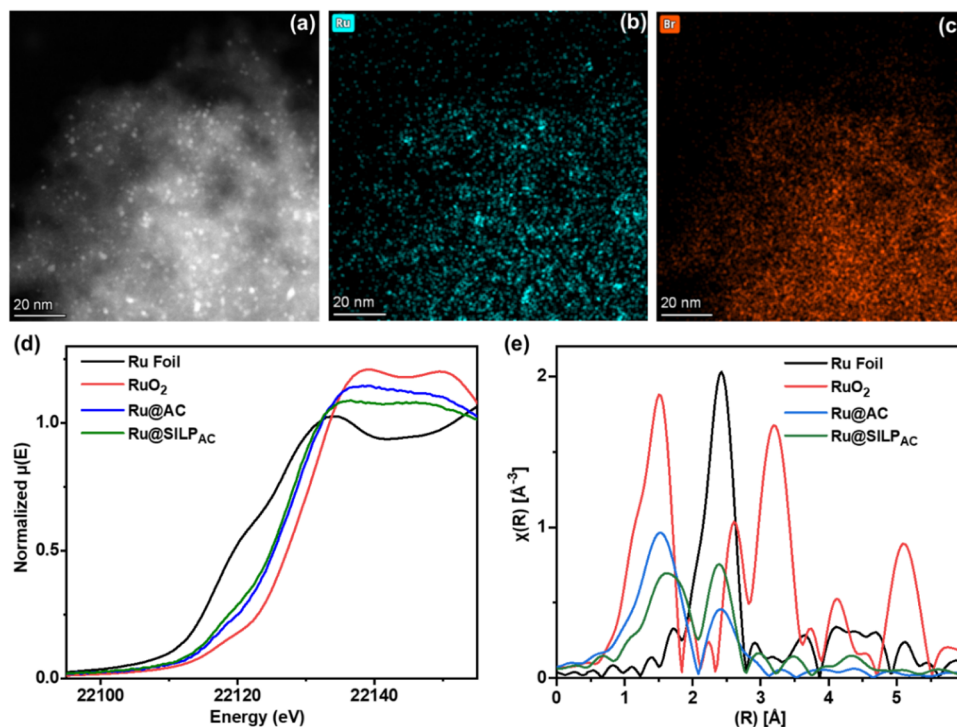
Figure 3. Characterization of Ru@SILP AC (1.1 mmol IL ·g -1 , 0.1 mmol Ru ·g -1 theoretical) by (a) HAADF-STEM, (b, c) HAADF-STEM-EDX elemental mapping images of (b) Ru L \alpha and (c) Br K \alpha , (d) normalized Ru K-edge X-ray absorption near edge structure (XANES) spectra of Ru@SILP AC and reference materials, and (e) k^2 -weighted R-space Fourier transformed extended X-ray absorption fine structure (FT-EXAFS) spectra of Ru@SILP AC and reference materials (without phase correction) and Ru foil with \chi(0.5) .
