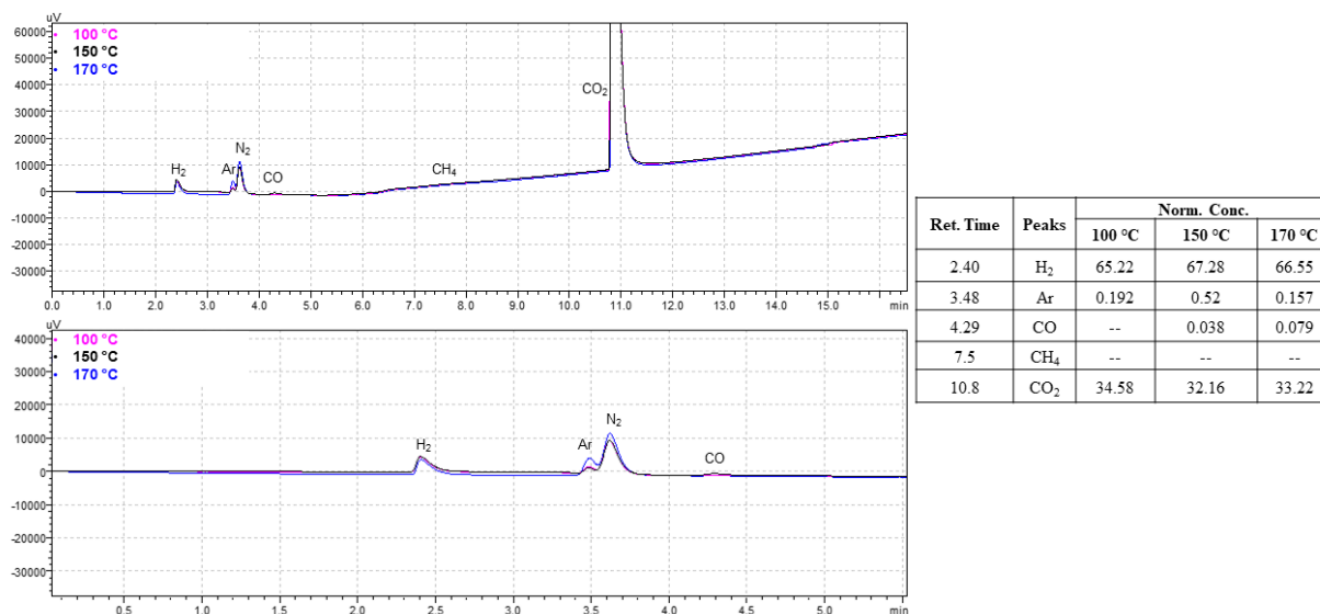
Figure S8. GC-TCD spectra and results for hydrogenation of CO 2 at different temperatures (100 °C, 150 °C, and 170 °C). Reaction Conditions: Ru@SILP AC (50 mg, 1.1 mmol L .g -1 , 0.1 mmol Ru .g -1 theoretical, 0.081 mmol Ru .g -1 experimental) under 60 bar total pressure with CO 2 :H 2 = 1:2 using solvent as NEt 3 (2.32 mL, 16.7 mmol) + H 2 O (0.88 mL, 48.8 mmol), total volume: 3.2 mL, NEt 3 /H 2 O molar ratio = 0.34, time: 1 h.
